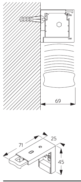
SG 8920 Bracket
