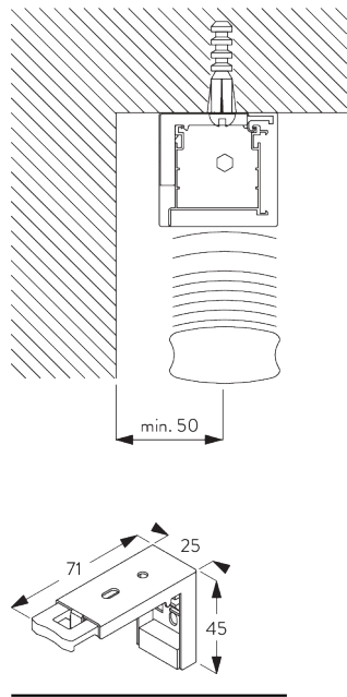
SG 8920 Bracket
