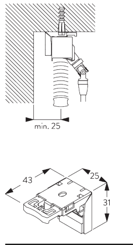
SG 10101 Bracket
