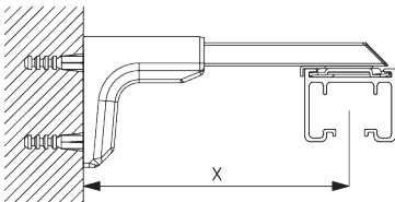
Universal Smart Fix SG 11154 - SG 11156 and clamp SG 3033 / SG 3044 Screw SG 11158 (M4x12) needed.
