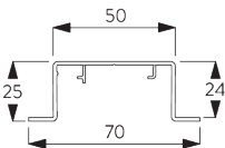
SG 2615 Recess profile
