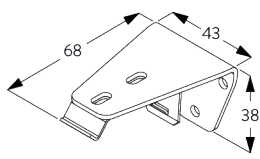
SG 2363 Bracket 68 mm
