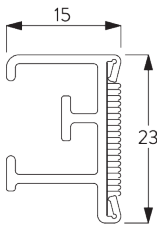
SG 2211 Velcro profile
