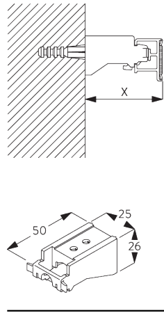
SG 3655 Bracket 50 mm
