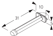
SG 10641 Side guide eyelet
