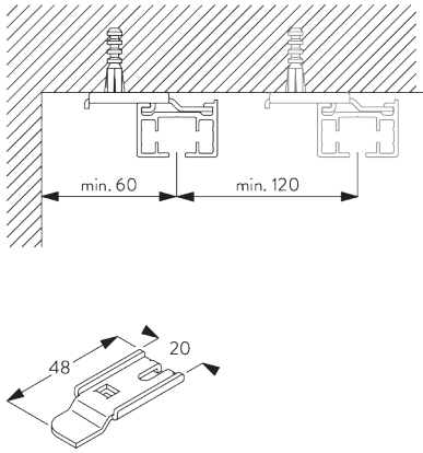
SG 3041 Bracket
