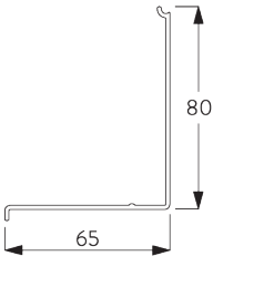
SG 10997 Box cover 90 mm
