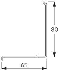
SG 10997 Box cover 90 mm
