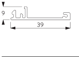
SG 11419 Side guide cover
