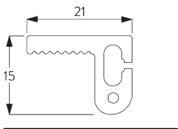
SG 11421 Zip profile
