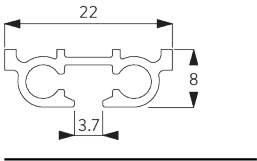
Profile and bending information
